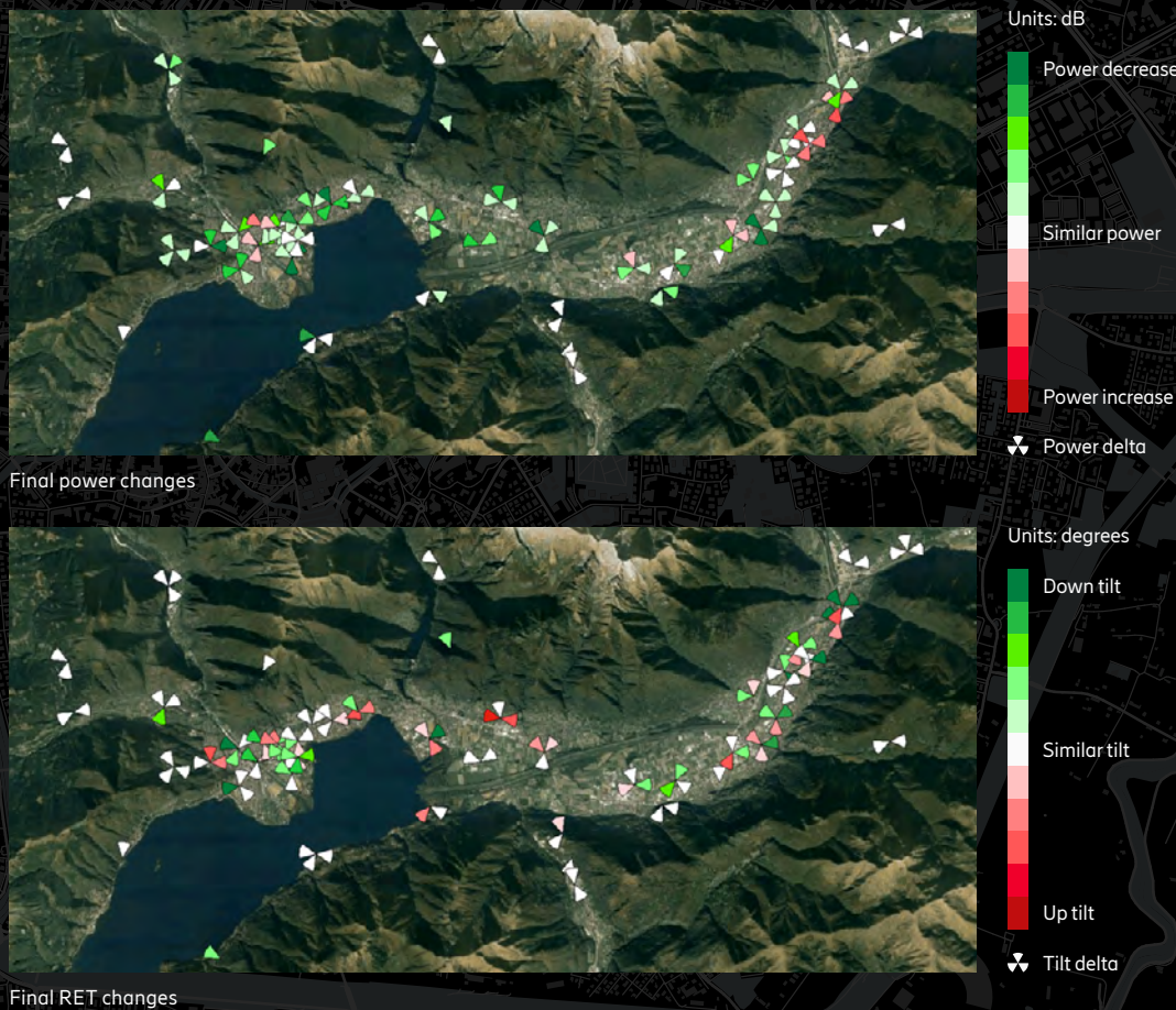
Figure 27: Power and RET changes in the Ticino area of Switzerland
